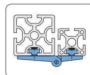
1 profile 60×60 1 profile 40×40
